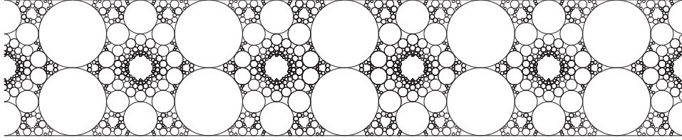
FIGURE 10. The strip cross section through the tangent point \mathbf{e}_2 + \mathbf{e}_3 and the center of the parallelepiped. The constraints are x_2 = x_3 and x_1 + x_4 = 0 .
