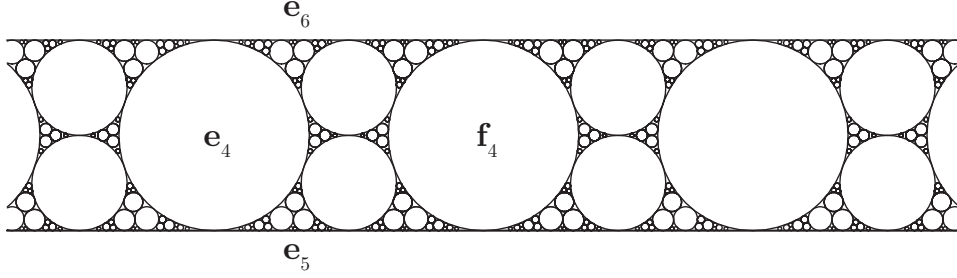
FIGURE 6. The cross section through the centers of H_{\mathbf{e}_4} and H_{\mathbf{f}_4} , and in a plane perpendicular to H_{\mathbf{e}_5} and H_{\mathbf{e}_6} .
