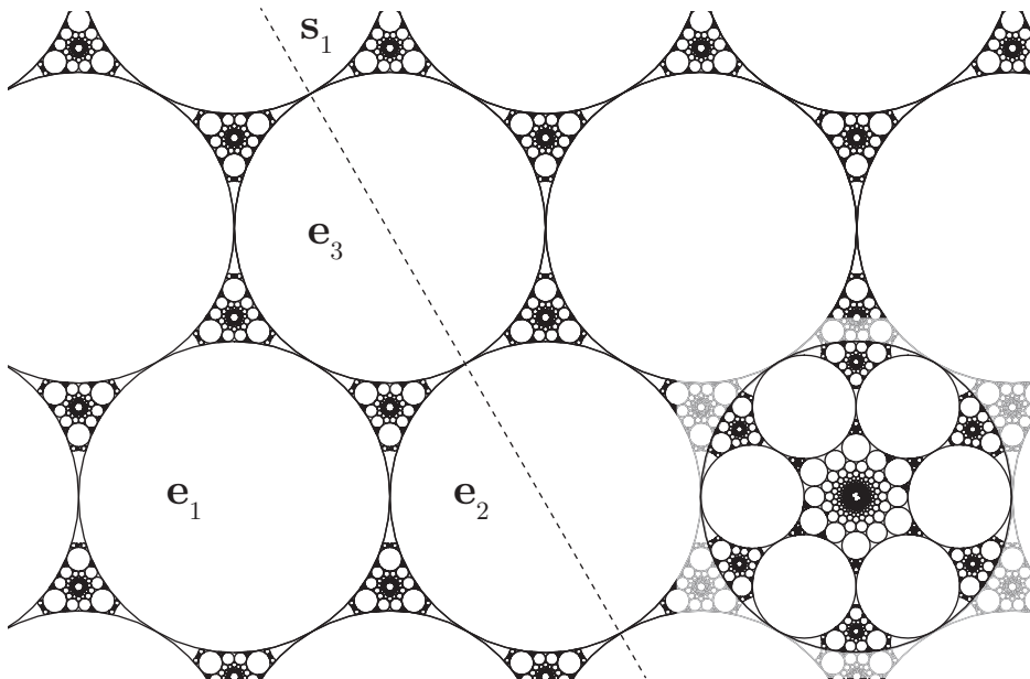
FIGURE 4. A cross section of the strip version of the sphere packing. The cross section goes through the centers of H_{e_1} , H_{e_2} , and H_{e_3} , and is parallel to the planes H_{e_4} and H_{e_5} . The dotted line represents H_{s_1} , and R_{s_1} restricted to this cross section is reflection through the dotted line. The lower right inset is the inverse of this packing in the circle at that position. It is the cross section of the sphere packing that appears in Soddy’s paper [Sod37, Figure 1].
