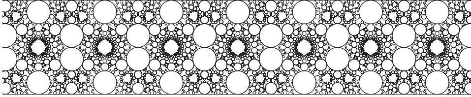
FIGURE 9. The strip cross section through the tangent points \mathbf{e}_1 + \mathbf{e}_4 and \mathbf{e}_2 + \mathbf{e}_3 . The constraints are x_1 = x_4 and x_2 = x_3 .
