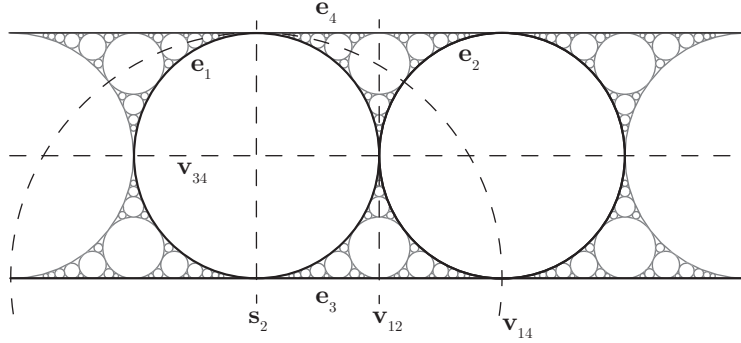
FIGURE 3. The strip packing and its symmetries.
