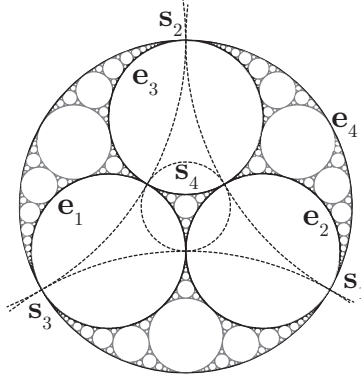
FIGURE 2. The circles of inversion (dotted lines) that generate the Apollonian packing. In this figure and figures throughout the paper, we will label a circle H_{\mathbf{n}} with its normal vector \mathbf{n} .
