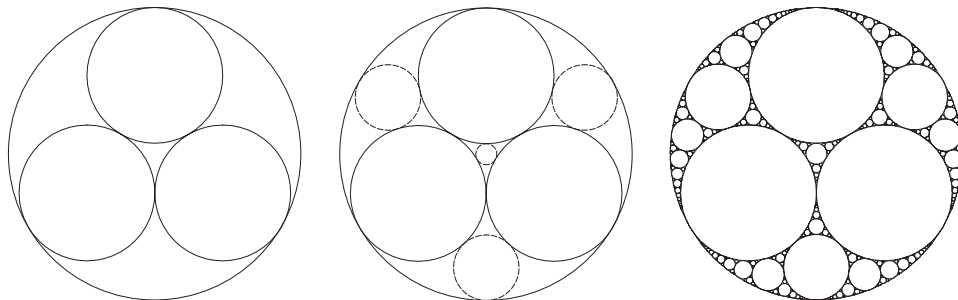
FIGURE 1. Generating the Apollonian packing.
