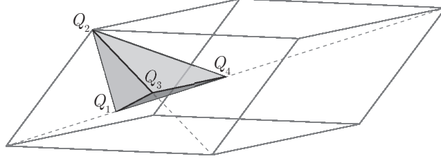
FIGURE 12. A parallelepiped that is the fundamental domain for G_1 , together with the tetrahedron Q_1Q_2Q_3Q_4 , which is a fundamental domain for G_2 .
