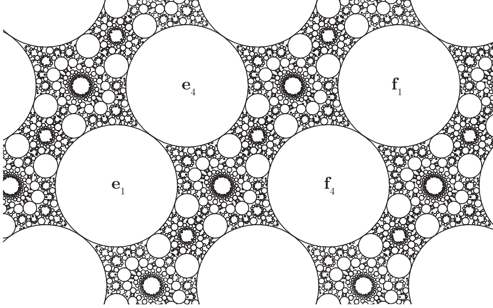
FIGURE 5. The cross section of the 4-dimensional strip version of the Apollonian packing (with E = \mathbf{e}_5 + \mathbf{e}_6 ), corresponding to x_2 = x_3 and x_5 = x_6 . The limit point of circles midway between H_{\mathbf{e}_1} and H_{\mathbf{f}_4} is the point \mathbf{e}_2 + \mathbf{e}_3 , which is where the hyperspheres H_{\mathbf{e}_2} and H_{\mathbf{e}_3} are tangent.
