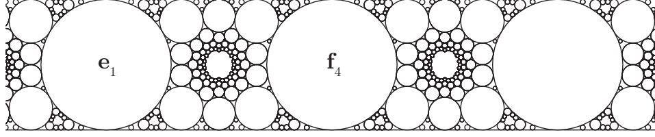
FIGURE 8. The strip cross section through the centers of H_{\mathbf{e}_1} and H_{\mathbf{f}_4} . It is a cross section of the sphere packing.
