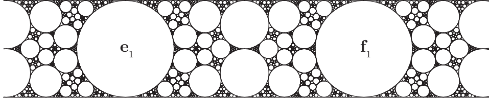
FIGURE 7. The cross section along the long diagonal of the parallelepiped and perpendicular to H_{\mathbf{e}_5} and H_{\mathbf{e}_6} .
