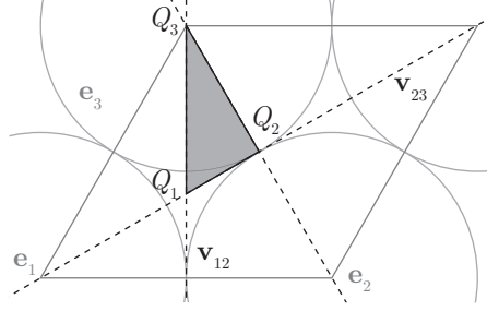
FIGURE 11. With \rho = 5 : A fundamental domain for G_2 (shaded triangle \Delta Q_1 Q_2 Q_3 ), inside a fundamental domain for G_1 (the parallelogram).
